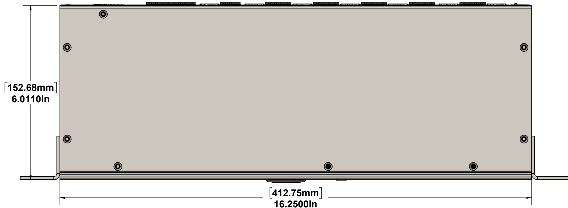
Top View
